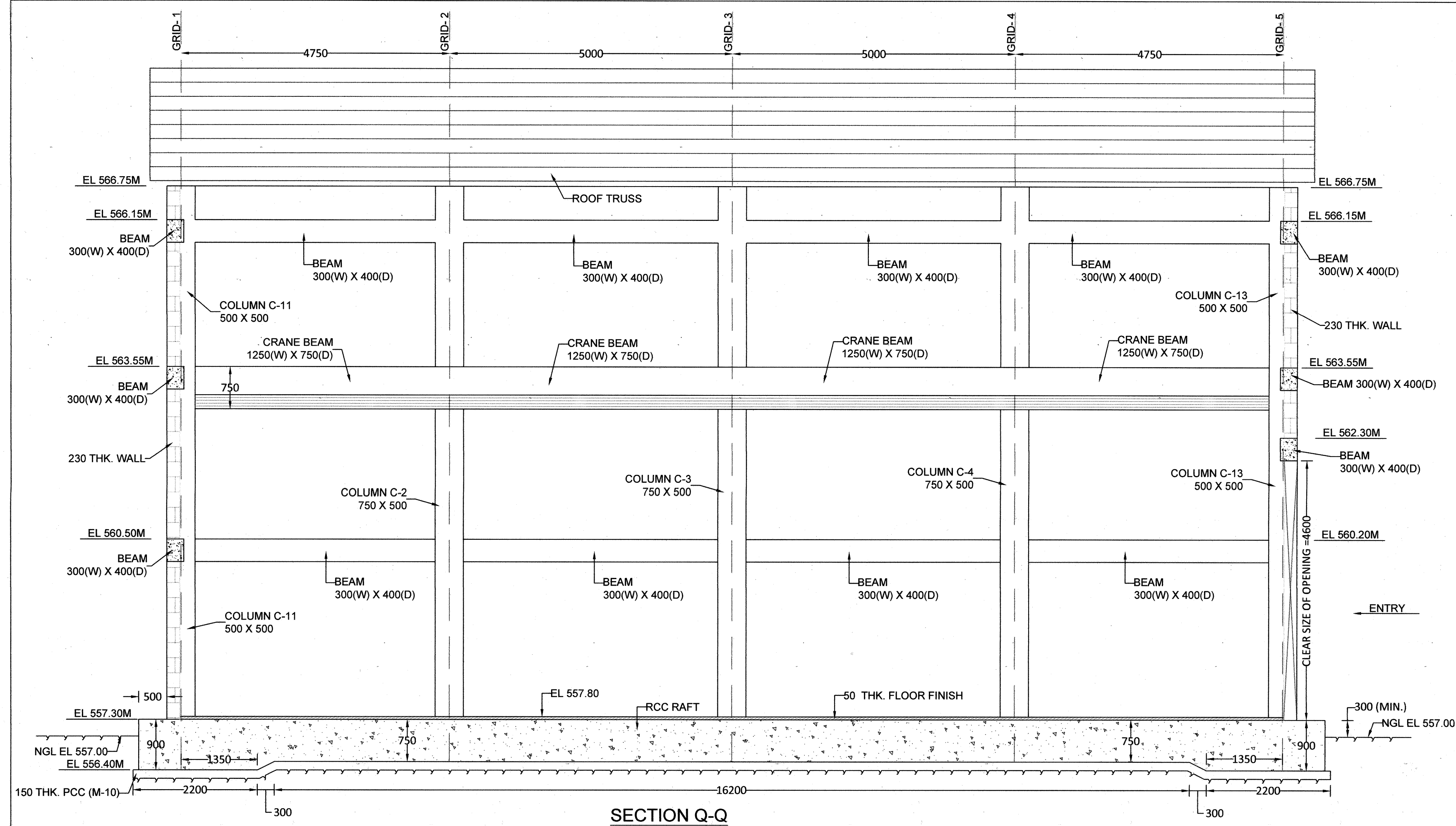
SECTION Q-Q
