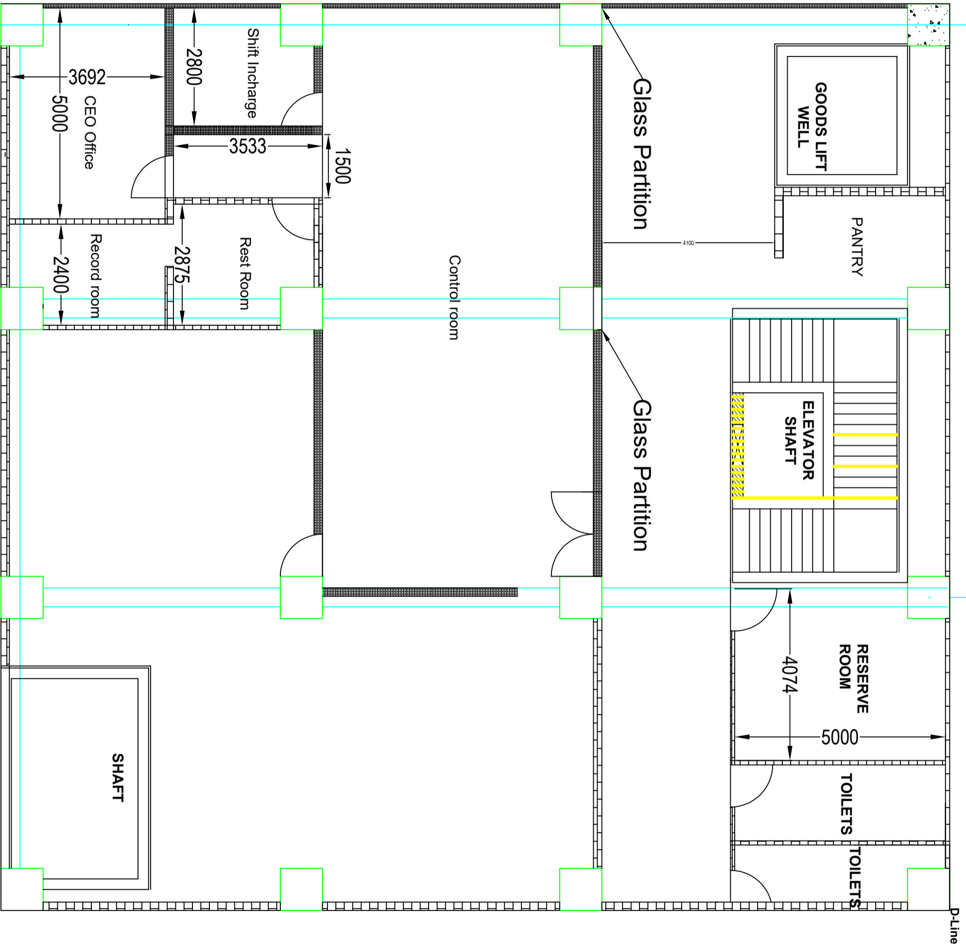
FLOOR PLAN FOR EL.543 M
