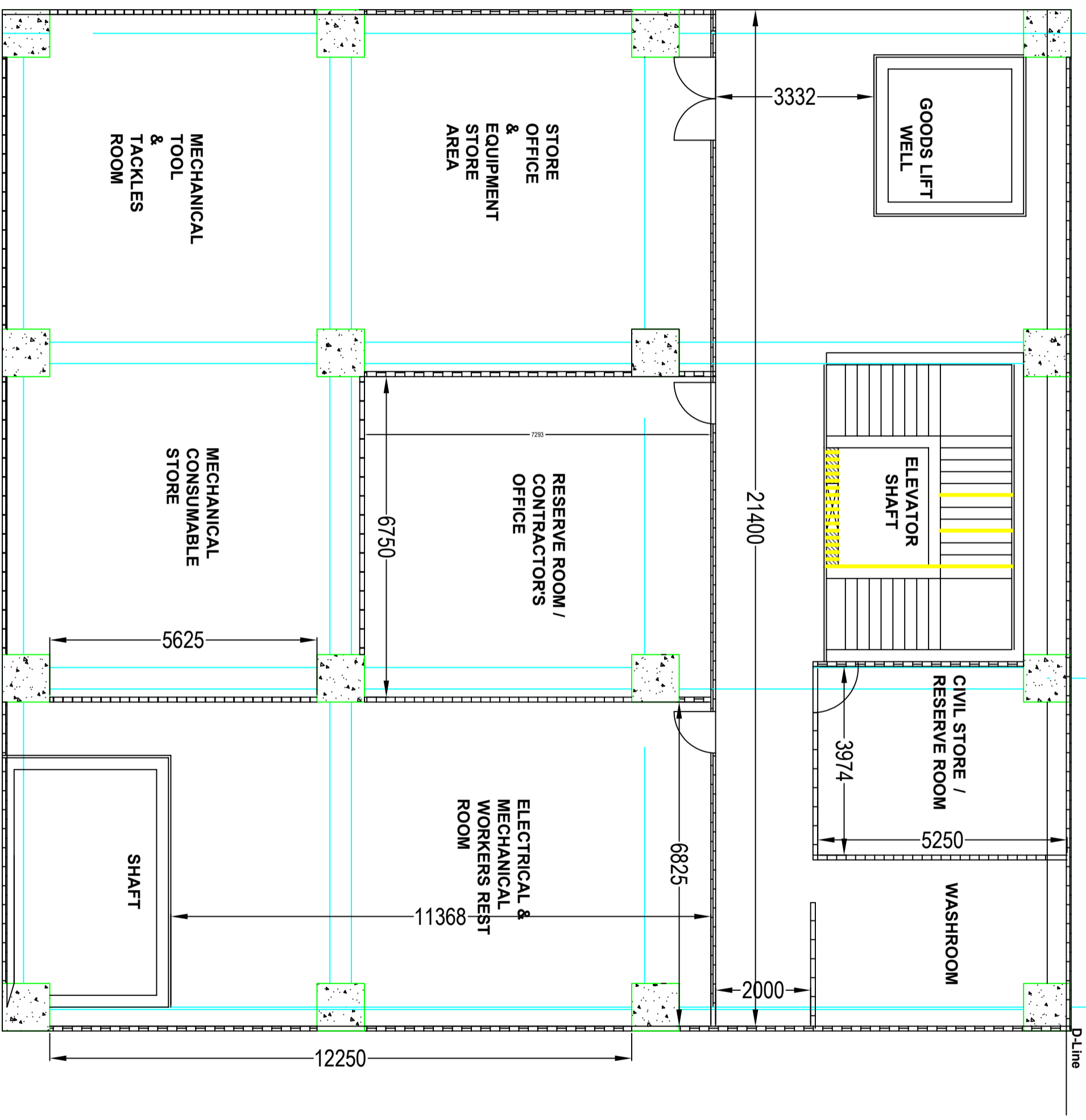
FLOOR PLAN FOR EL.523 (MIV Floor)
