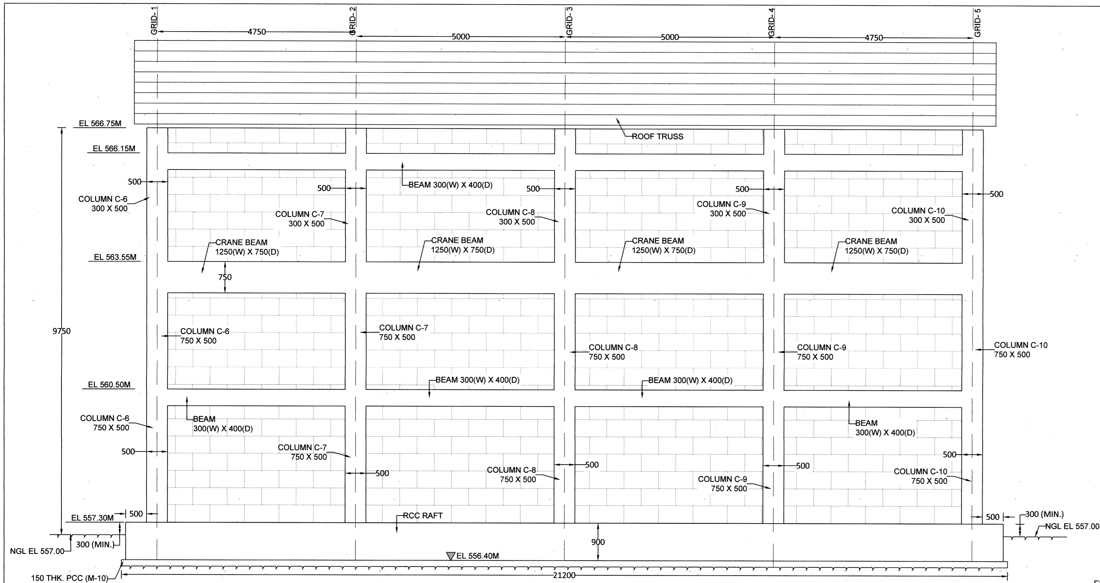
VIEW "3"
