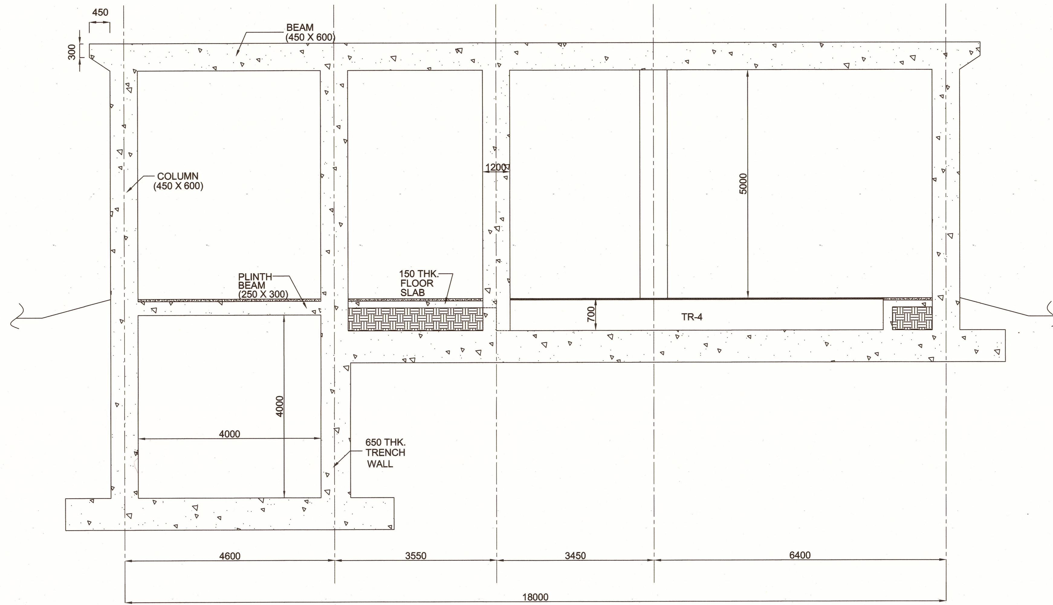
SECTION B-B
