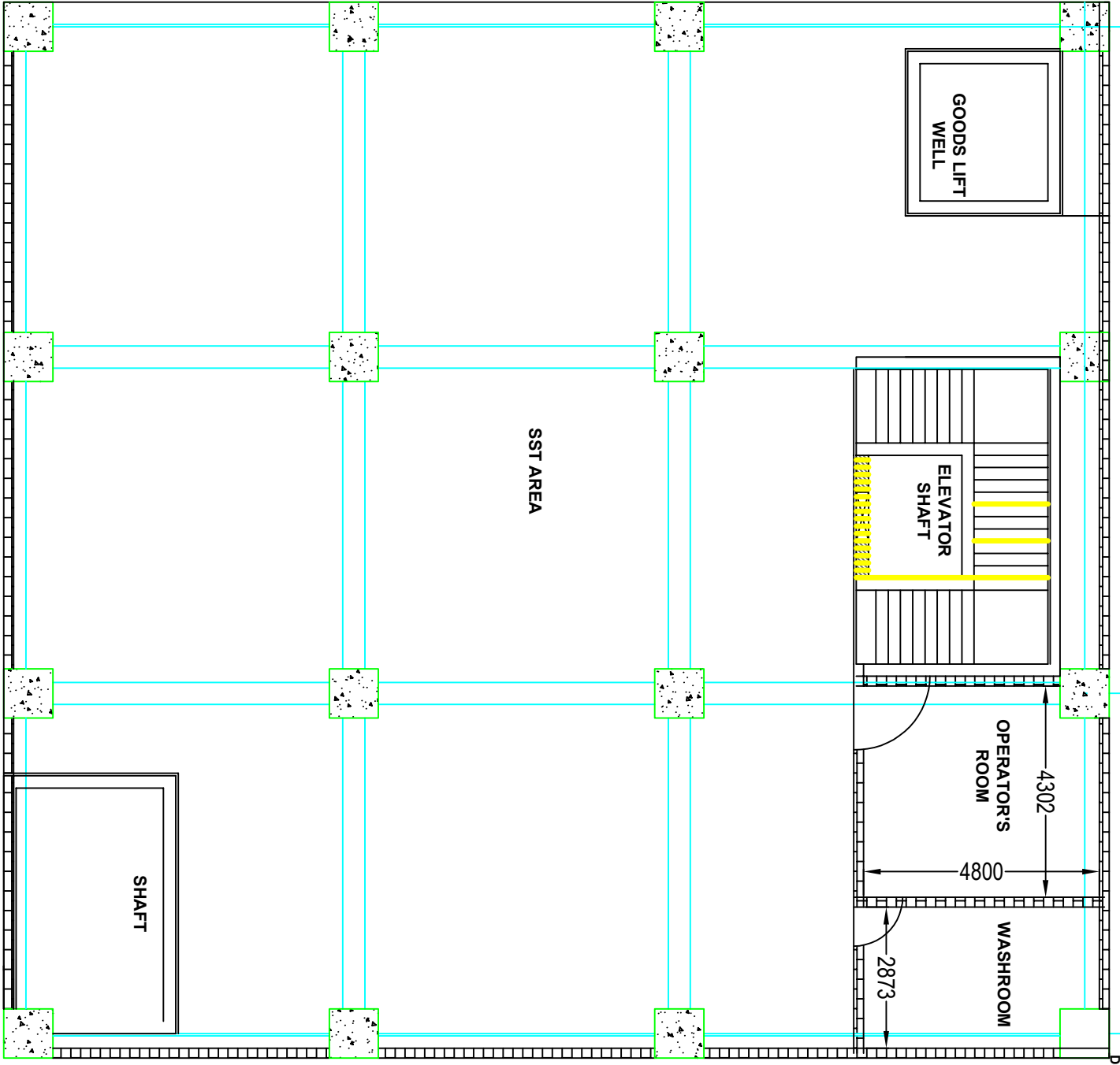
FLOOR PLAN FOR EL.534 (Generator floor )
