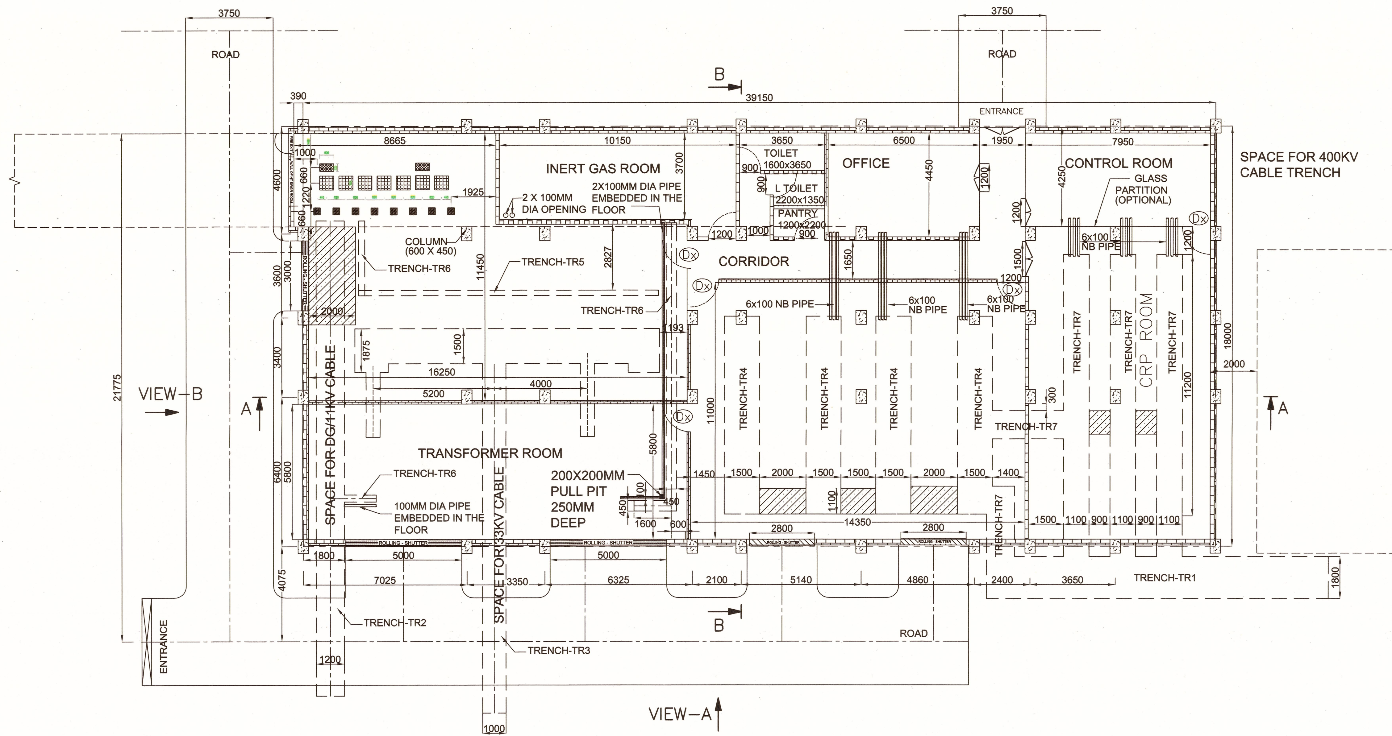
CONTROL ROOM BUILDING LAYOUT PLAN
