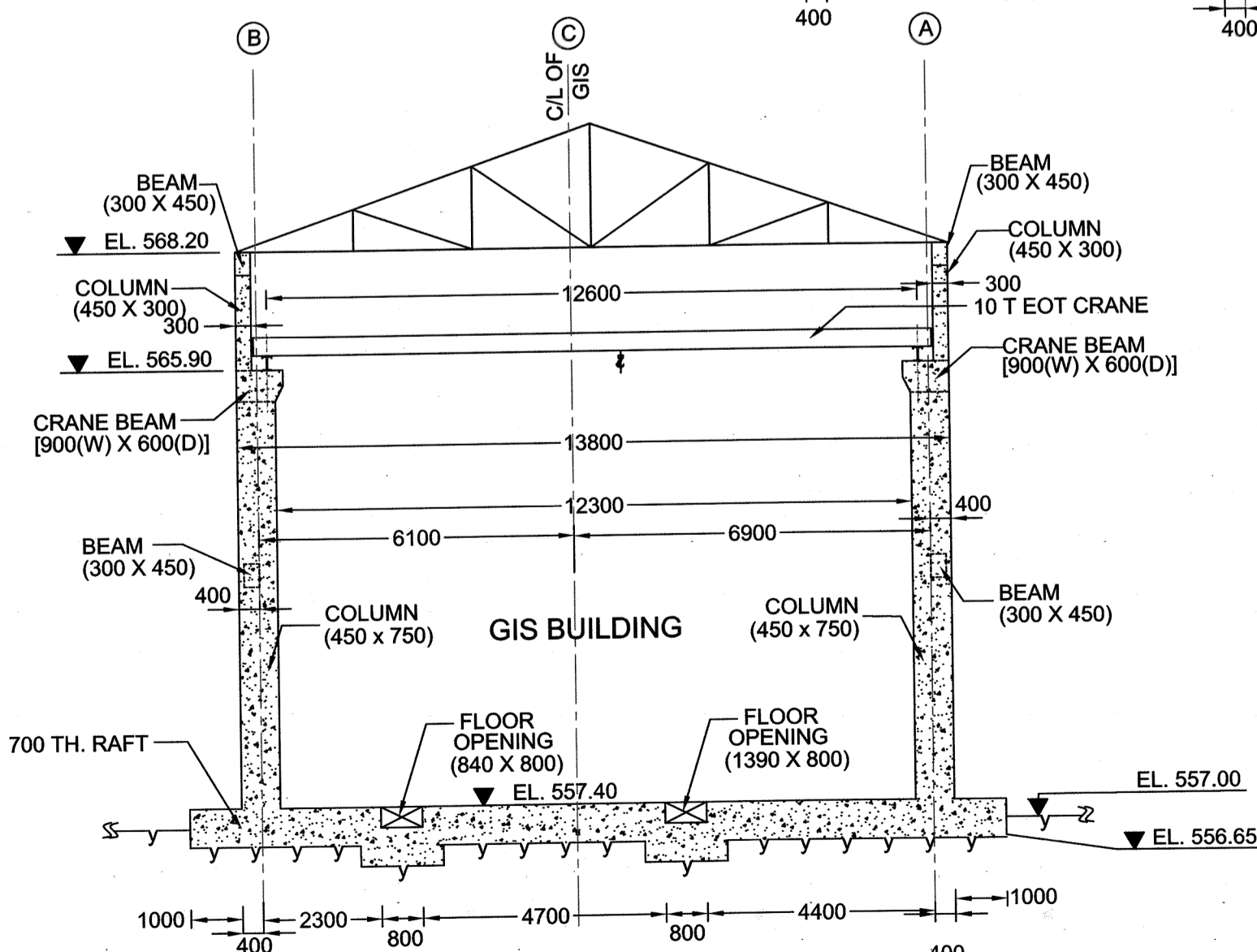
▲ SECTION 6-6
