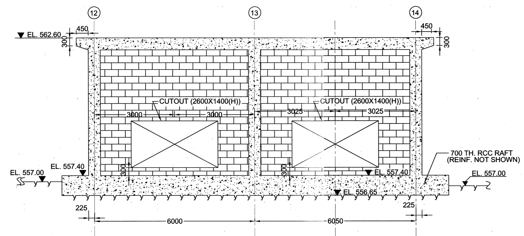
SECTION G-G
