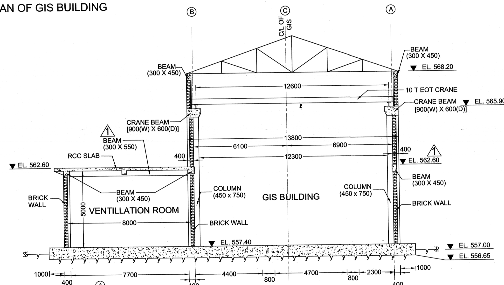
▲ SECTION 12-12
