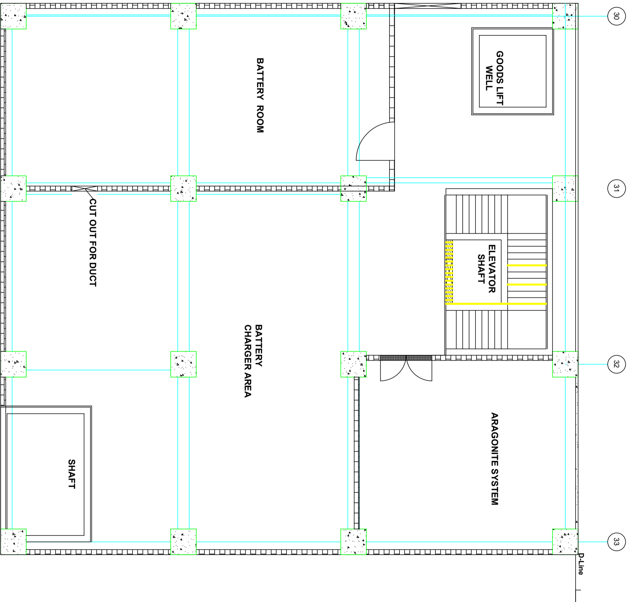
FLOOR PLAN FOR EL.547.8 (Battery Room)
