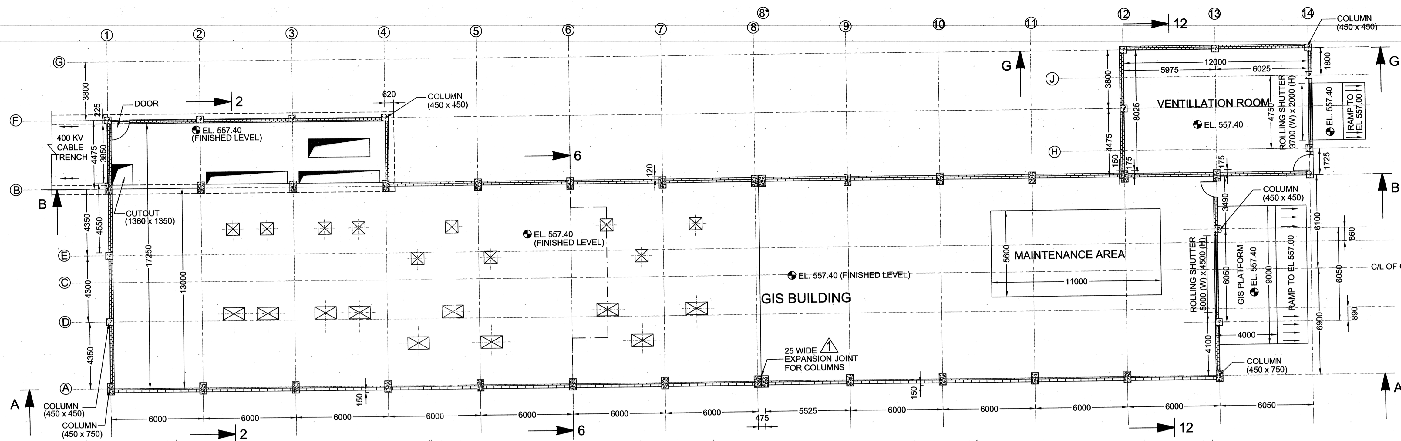
▲ LAYOUT PLAN OF GIS BUILDING
