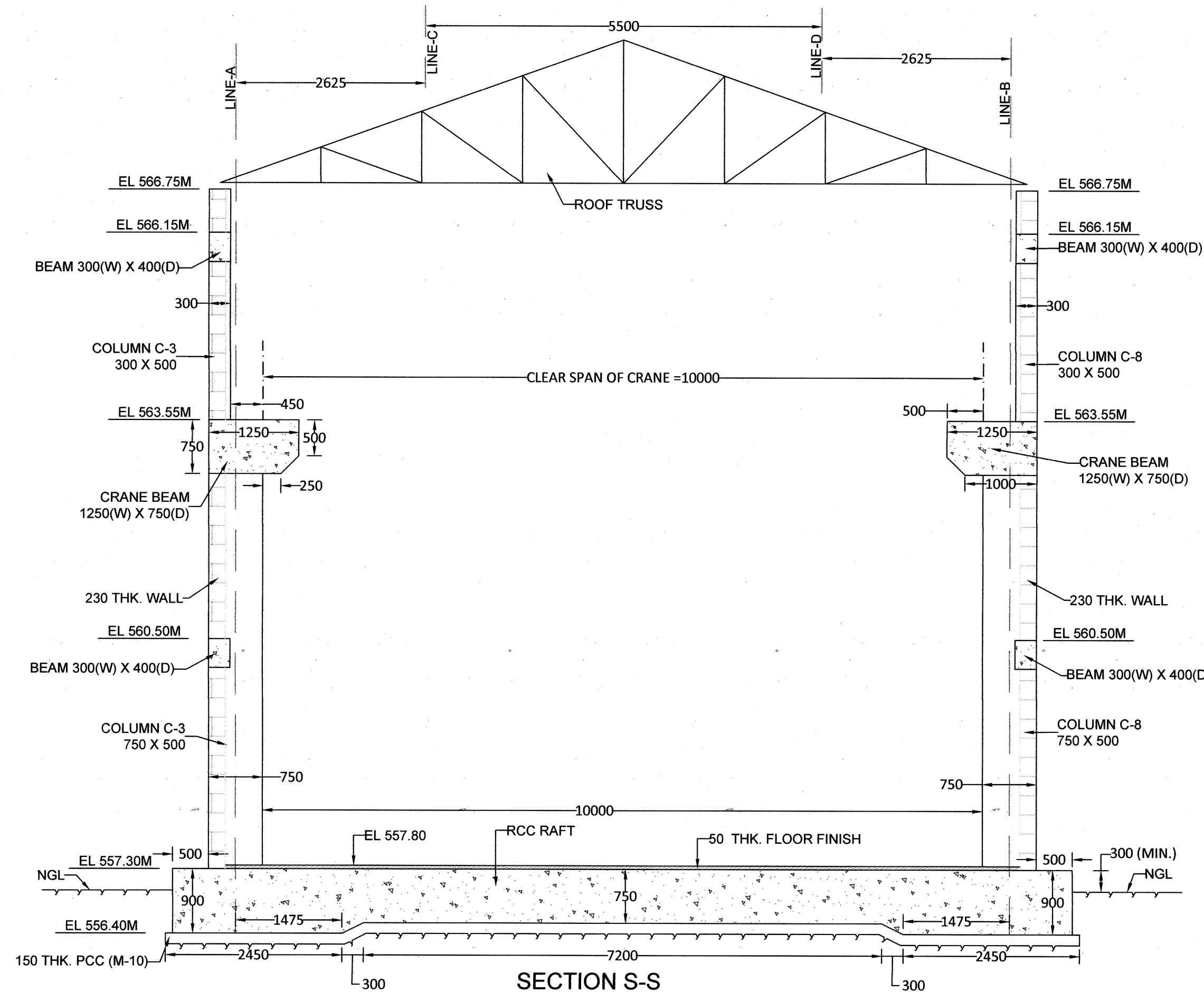
SECTION S-S
