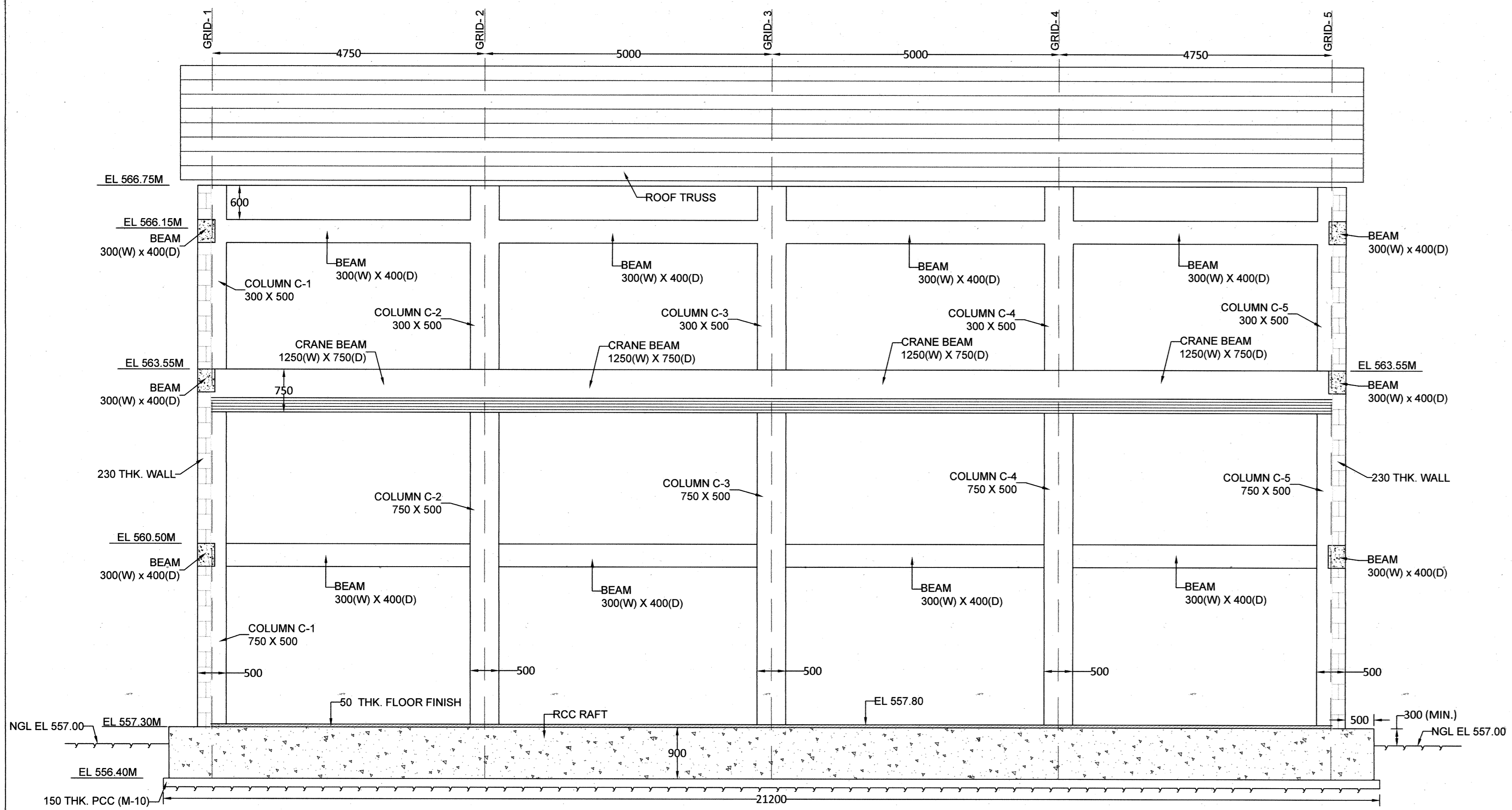
SECTION P-P
