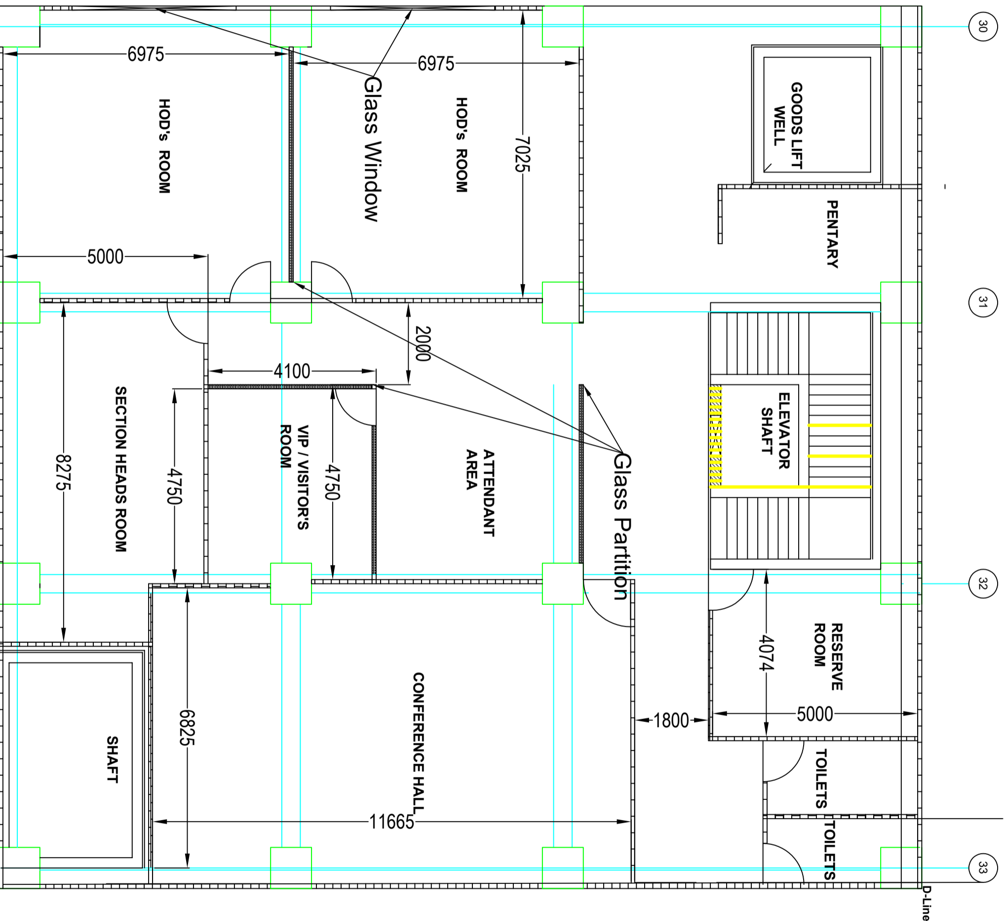
FLOOR PLAN FOR EL539 (Office)
