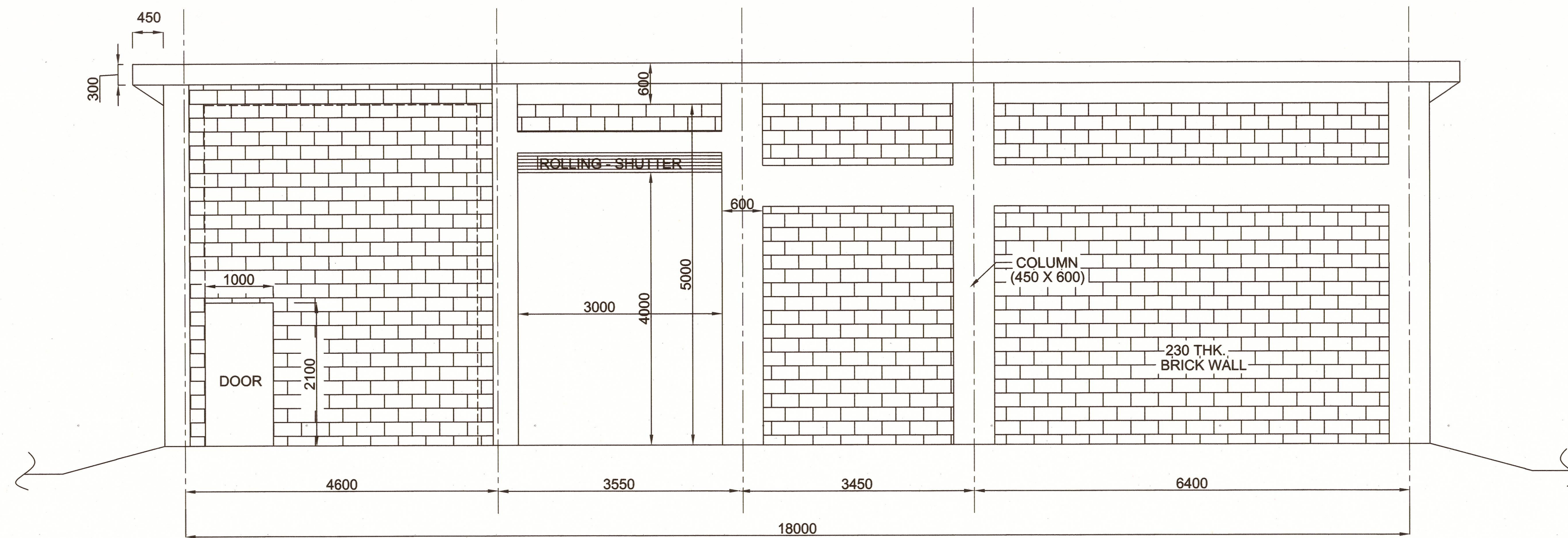
VIEW-B
