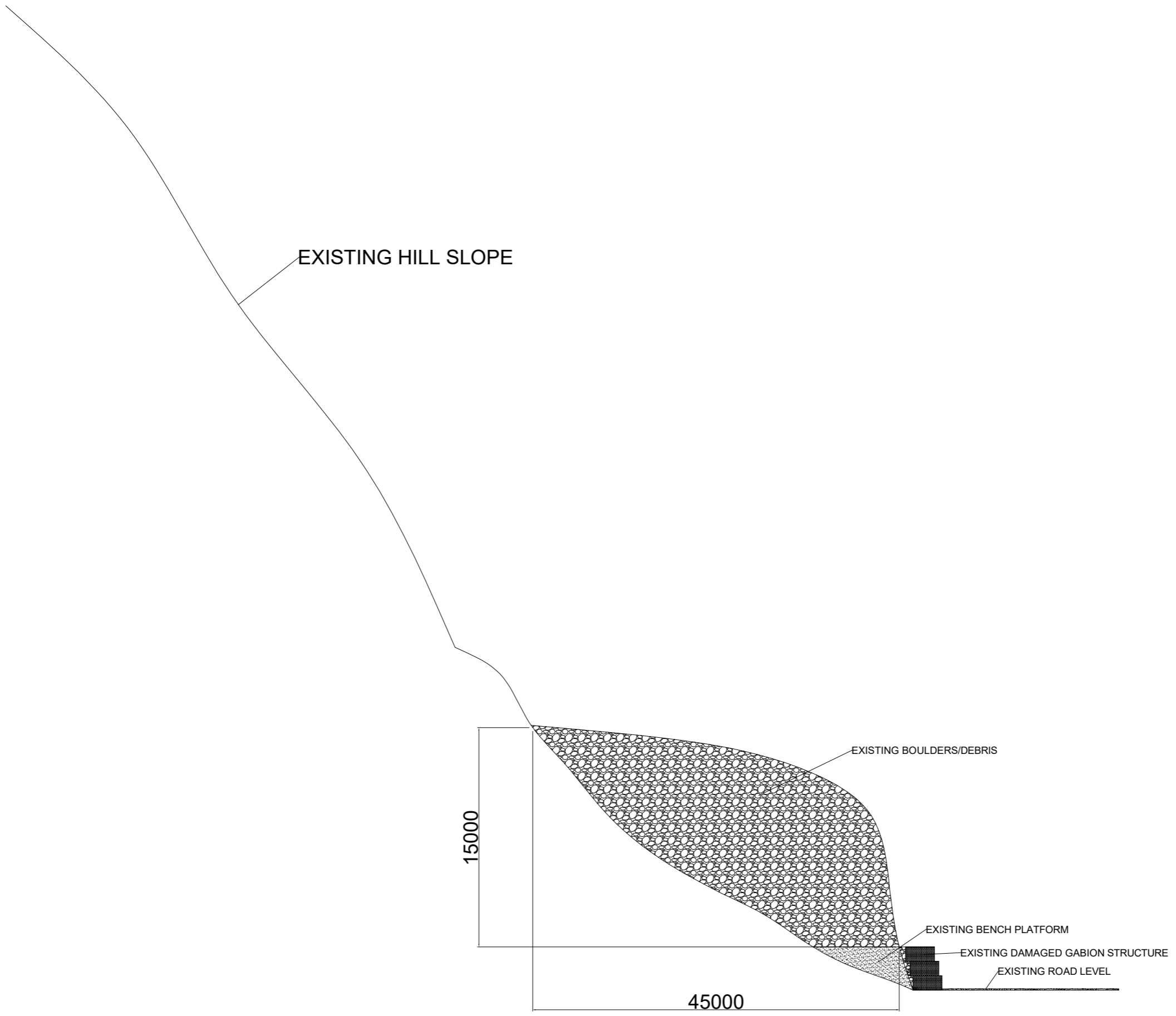
TYPICAL X-SECTION OF EXISTING HILL SLOPE AND DEBRIS ACCUMULATION FROM RD 160.00 TO 290.00M
