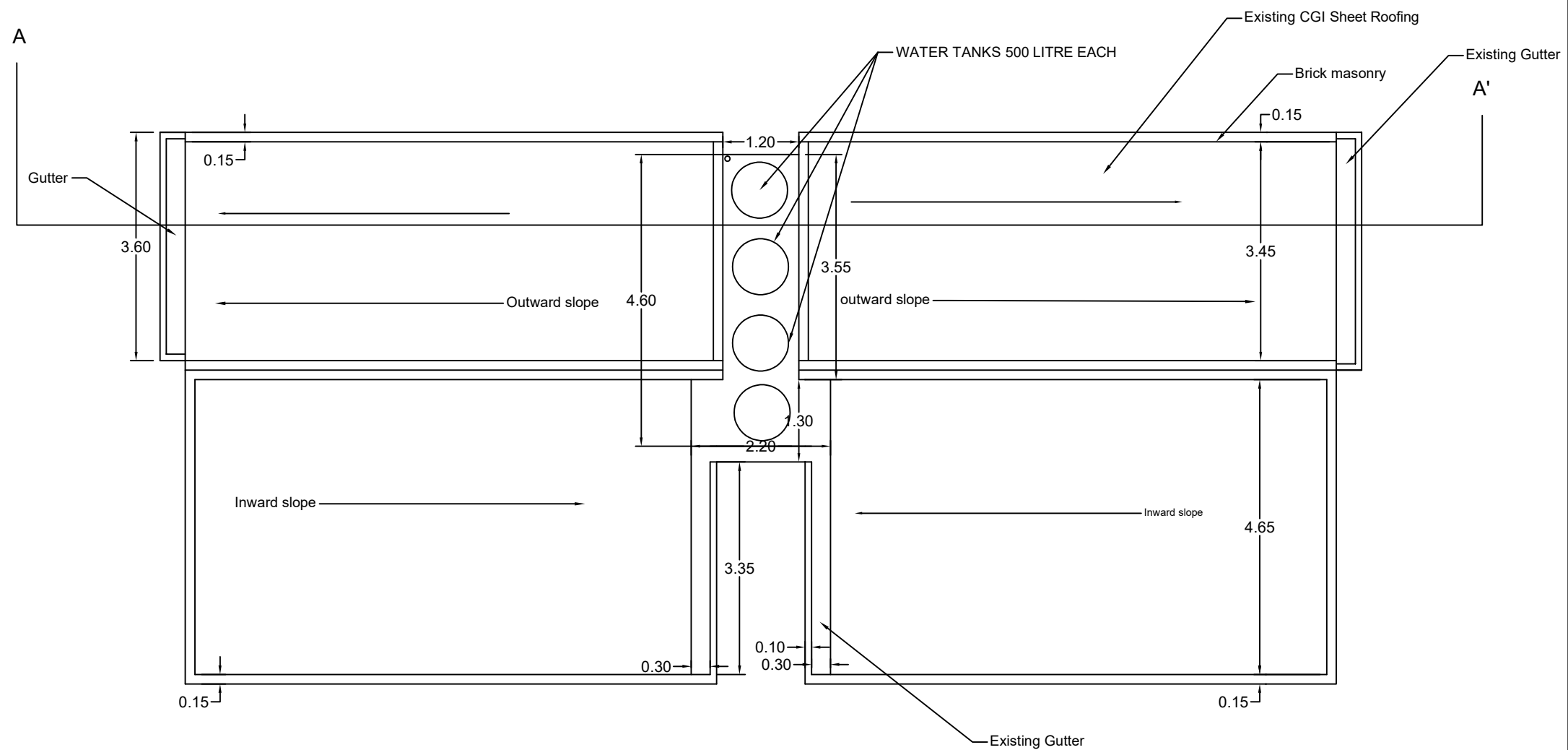
ROOF PLAN OF TYPE-III BLOCK 01 TO 6(2 storey)
