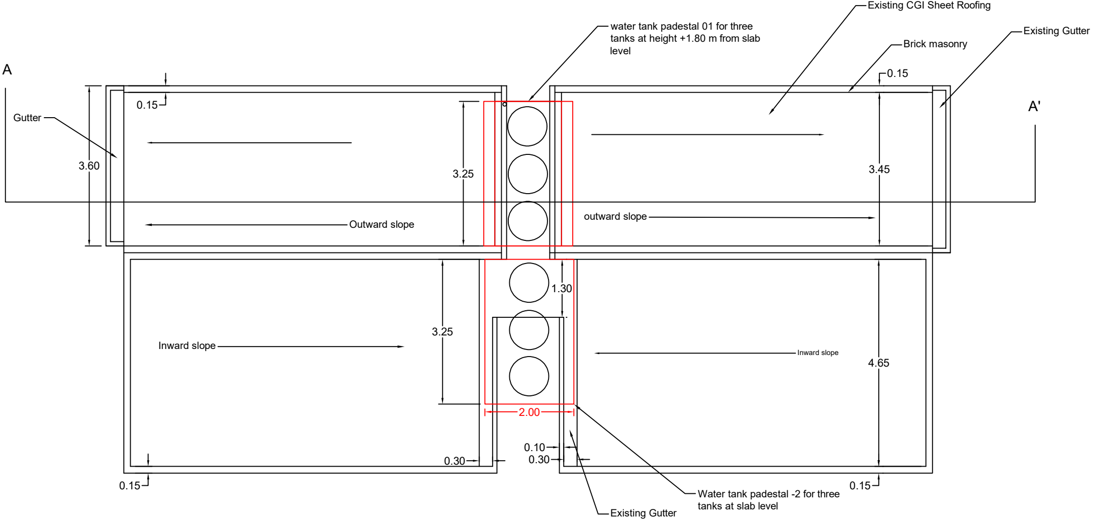
ROOF PLAN OF TYPE-III BLOCK 7 & 8( Three storey)
