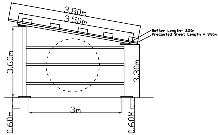
OIL TANK SHED
