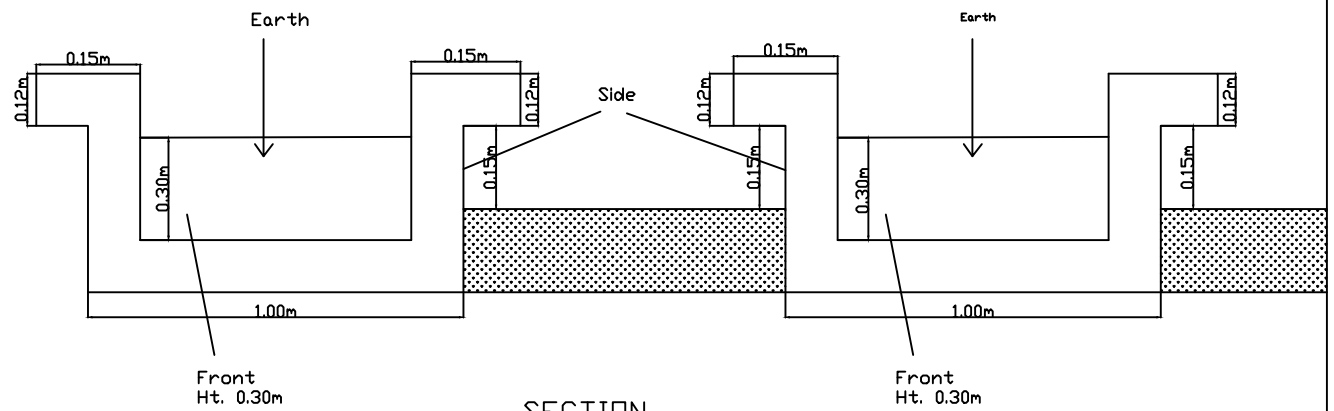
SECTION
