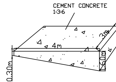
PLATFORM FOR OIL TANK SHED
