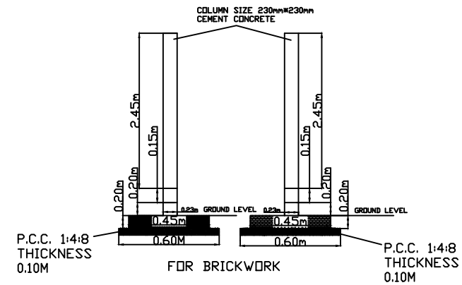
ELEVATION X,X'
