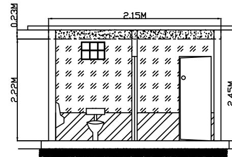
ELEVATION X,X'
