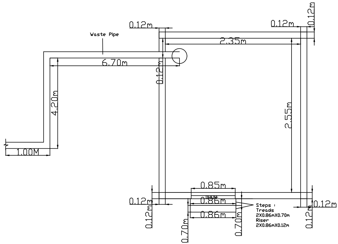
SHOWER ROOM ATTACH TO BATTERY ROOM
