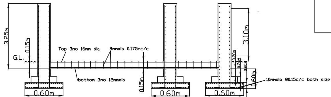
REINFORCEMENT DETAIL
